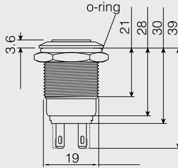
11mm Thread
