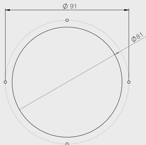
Fitting Hole Dimensions
