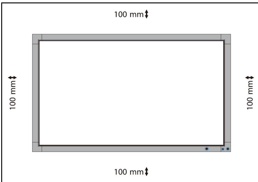
Figure 5 Ventilation Area
